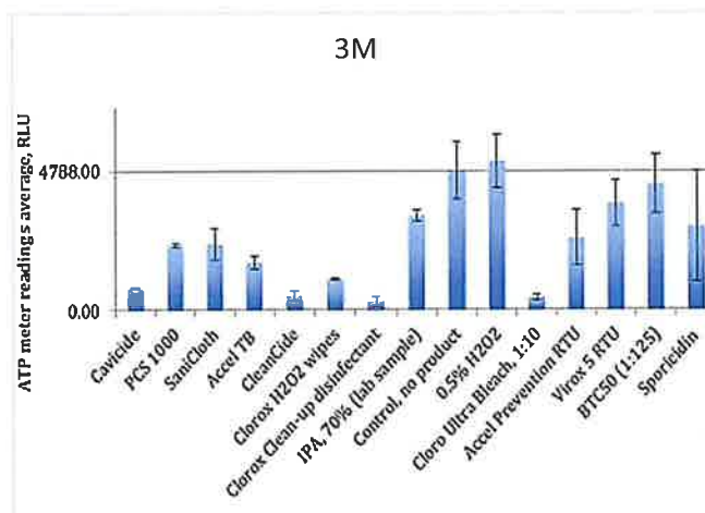
Figure 2. Interference of disinfectants on ATP measurements.
