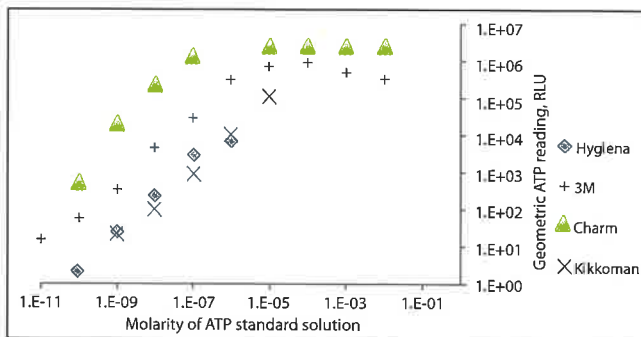
Figure 1. Testing showed ATP measurements from four different meters were linear at low concentrations but expressed lack of sensitivity and a flattened response at high concentrations.
